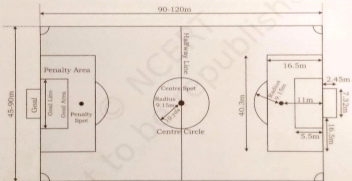
Fig. 6.16: Specifications of football ground
